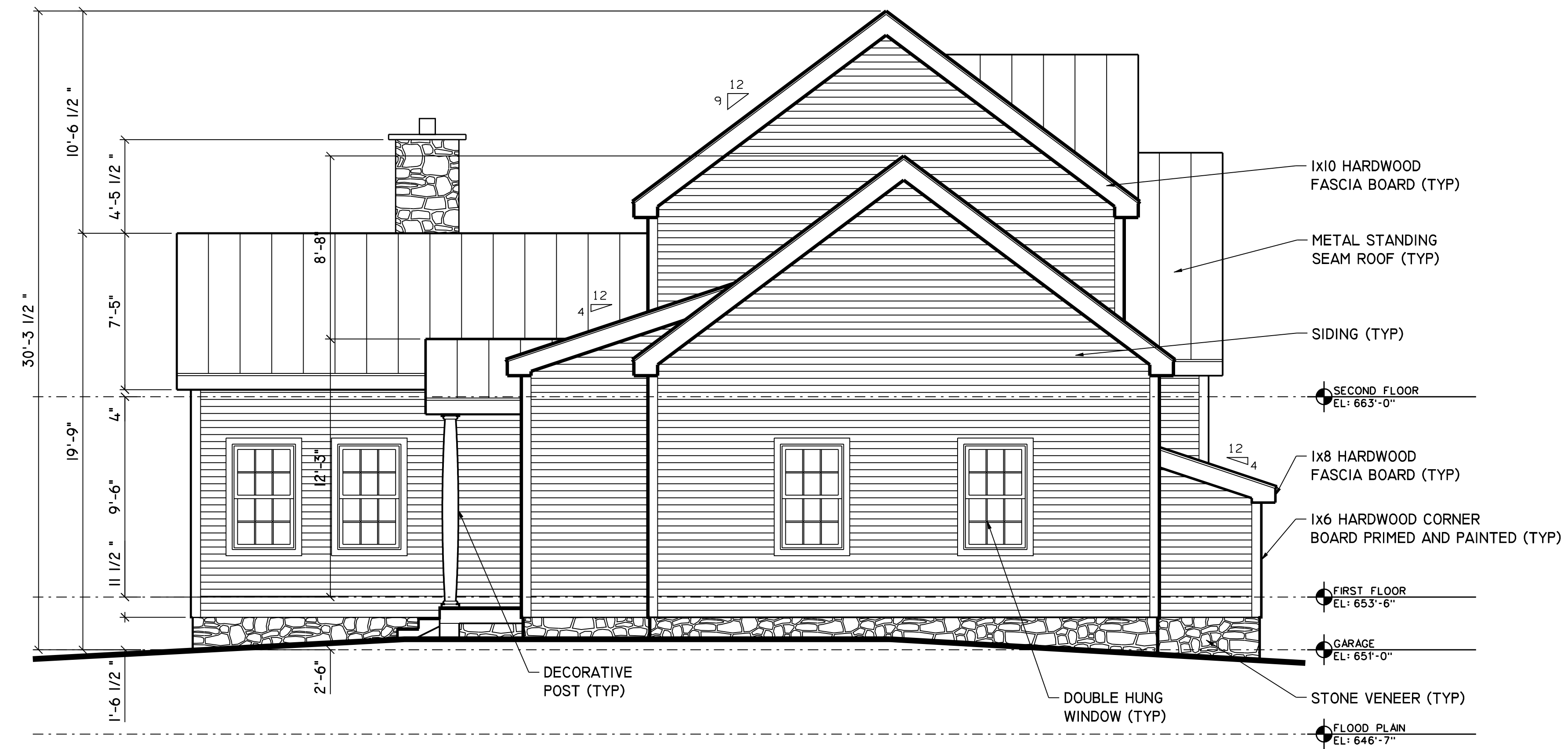
TYPICAL BUILDING SIDE ELEVATION Scale: 1/4" = 1'-0"
